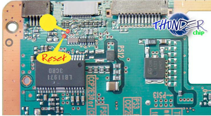
THUNDER chip pinout
