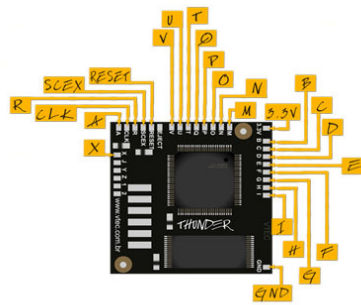
THUNDER chip pinout
